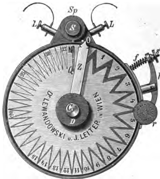
Graphite dial rheostat.
